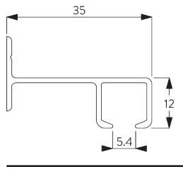
SG 6021p Profile
